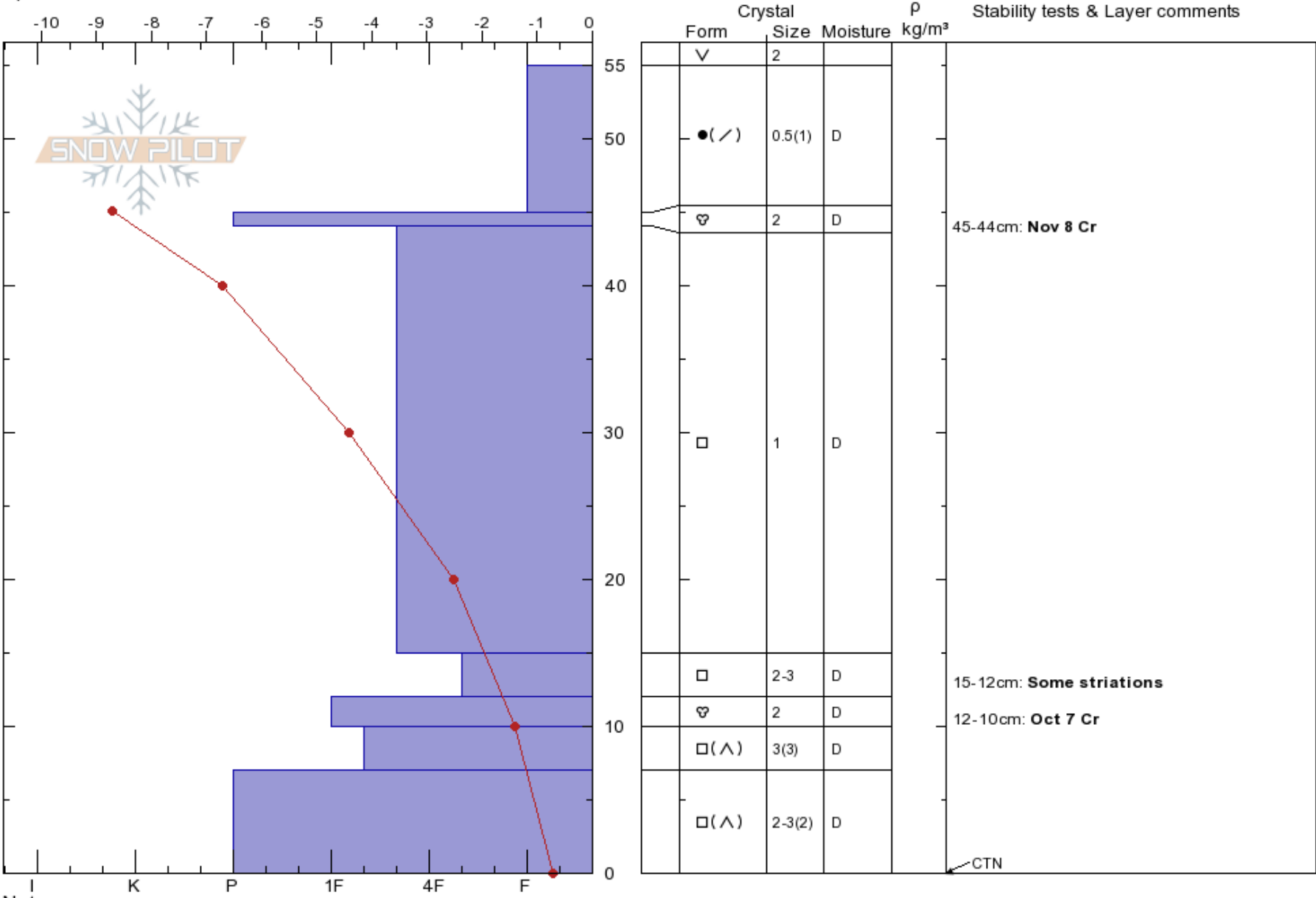
Notes: Sunshine ski hill Snow Study Plot.
